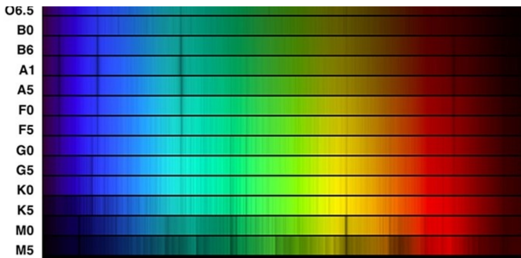
Figure 3: Spectra of Stars with Different Spectral Classes. This image compares the spectra of the different spectral classes. The spectral class assigned to each of these stellar spectra is listed at the left of the picture. The strongest four lines seen at spectral type A1 (one in the red, one in the blue-green, and two in the blue) are Balmer lines of hydrogen. Note how these lines weaken at both higher and lower temperatures, as Figure 2 also indicates. The strong pair of closely spaced lines in the yellow in the cool stars is due to neutral sodium (one of the neutral metals in Figure 2). (Credit: modification of work by NOAO/AURA/NSF)
