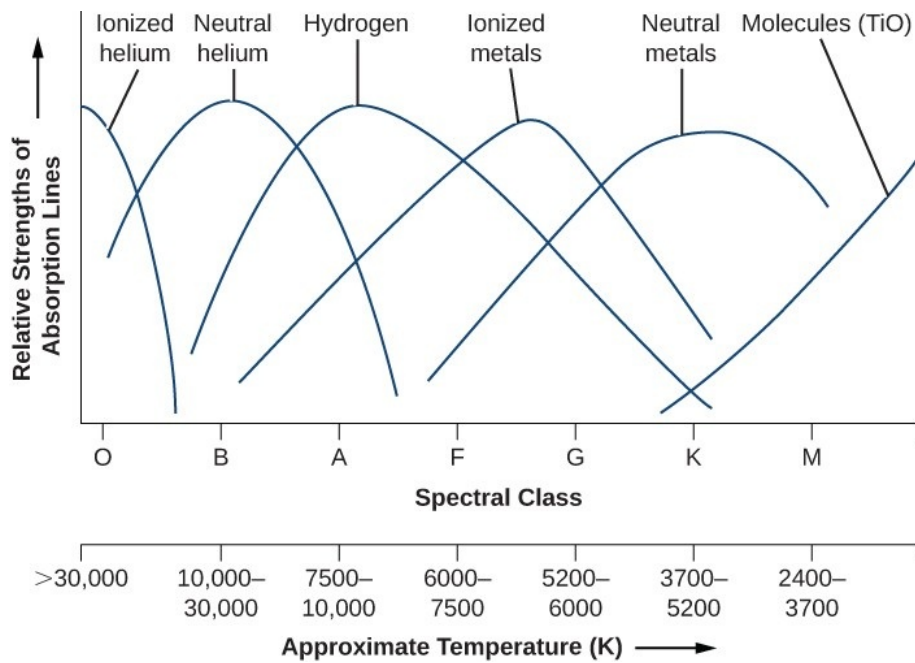
Figure 2: Absorption Lines in Stars of Different Temperatures. This graph shows the strengths of absorption lines of different chemical species (atoms, ions, molecules) as we move from hot (left) to cool (right) stars. The sequence of spectral types is also shown.
